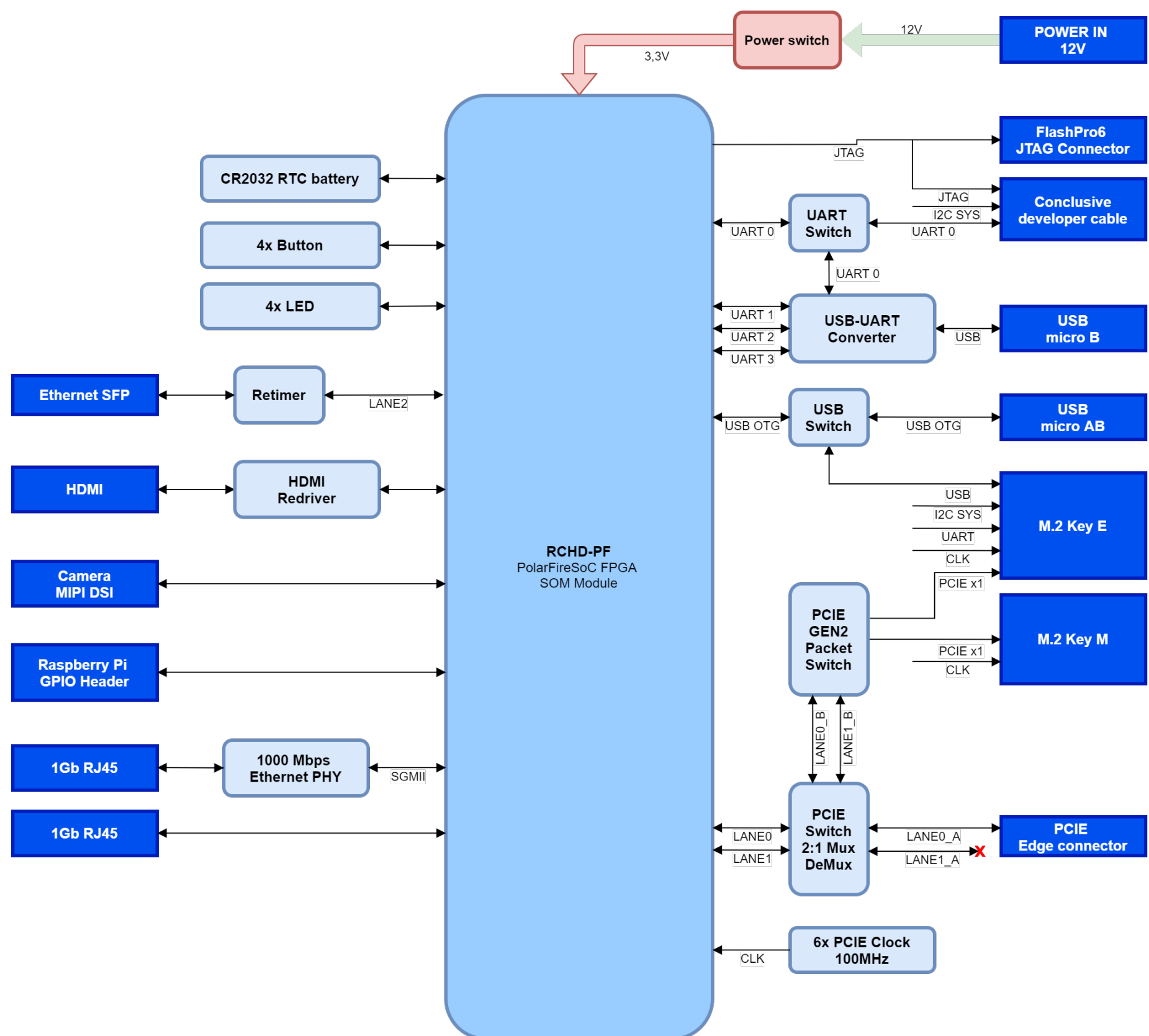
Fig. 5.1 Conclusive Engineering RCHD-PF-EVAL module block diagram.
