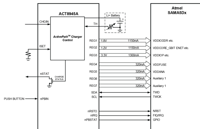
Fig. 6.4 ACT8945A PMIC block diagram and connectivity to ATSAM5D27 SoC.
