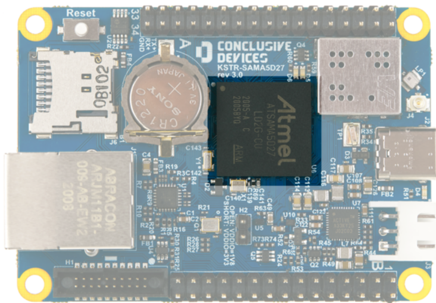
Fig. 6.1 ATSAMA5D27 SoC location
